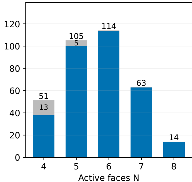
K=4: 347 closed states
