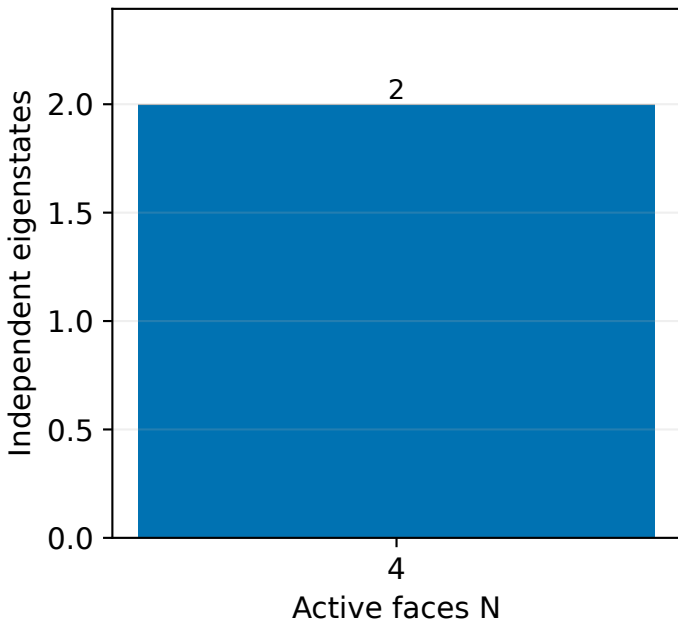
K=2: 2 closed states
