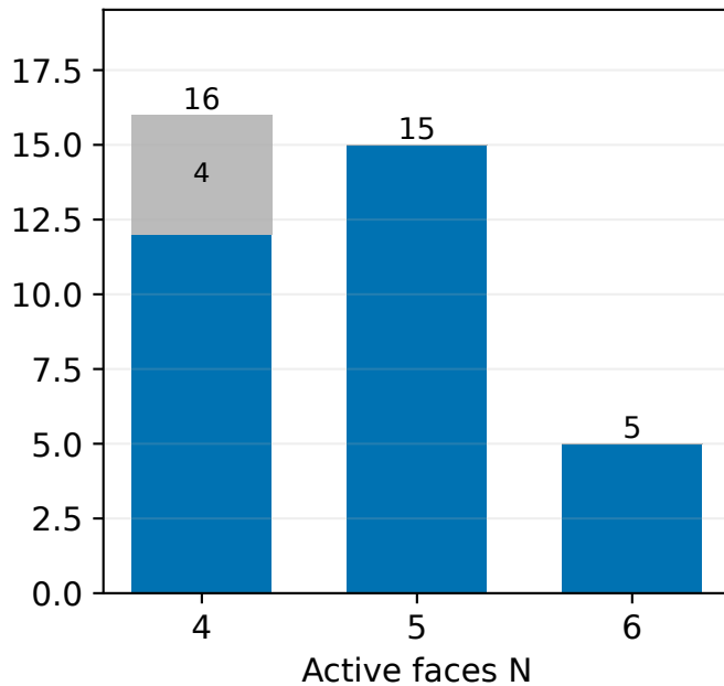
K=3: 36 closed states
