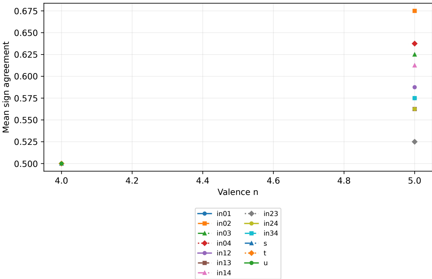
Local-chirality pilot: agreement over sampled planes
