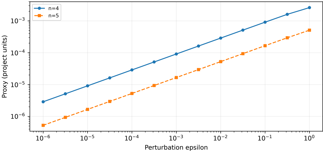
Imaginary perturbation: signed-mean proxy
