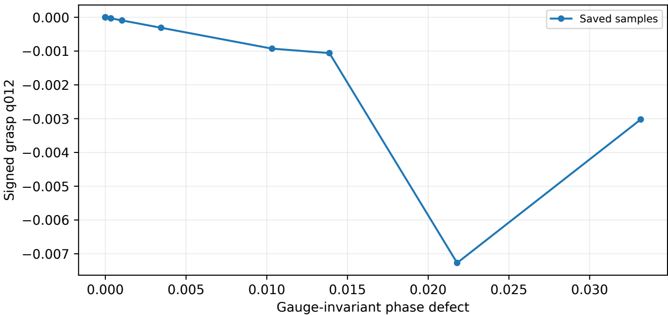
Cocycle-phase pilot
