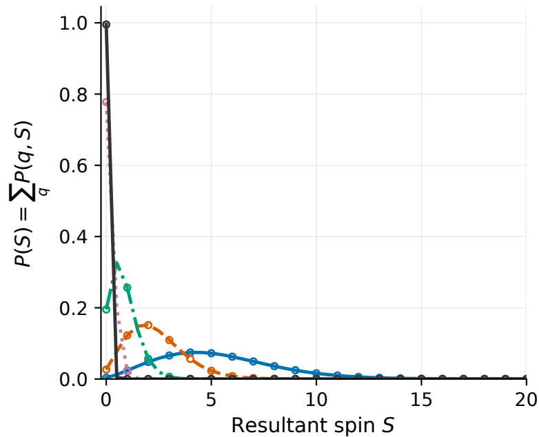
Ordinary per-copy total spin
