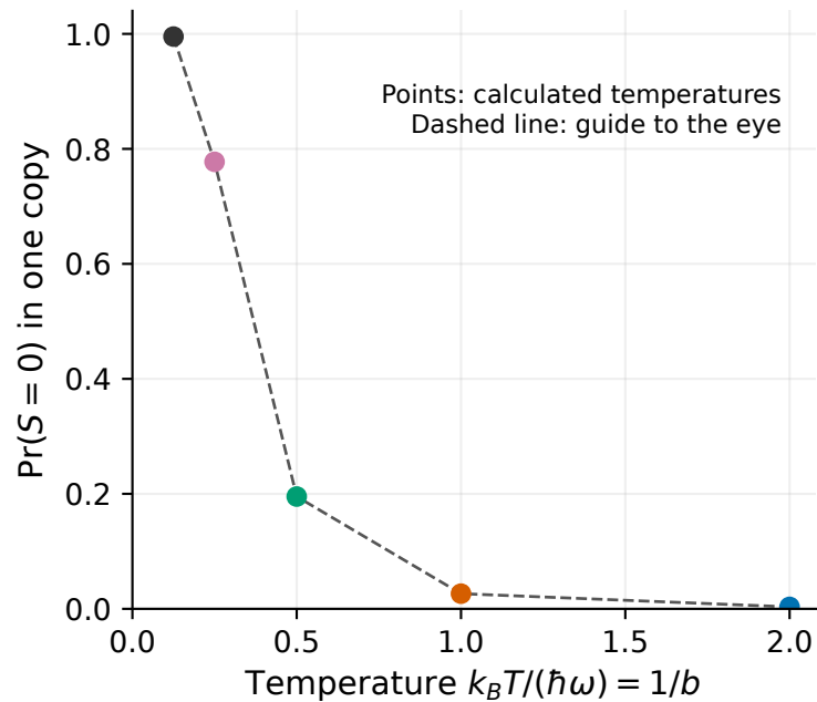
Probability of separate closure
