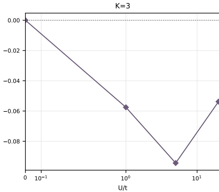
Graph dependence of the ground-state energy
