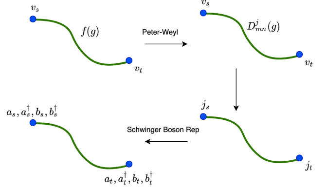
FIG. 7. Illustration of steps leading from cylindrical functions of edge holonomies to Schwinger Boson basis with pairs of ladder operators assigned to the source and target vertices respectively.
