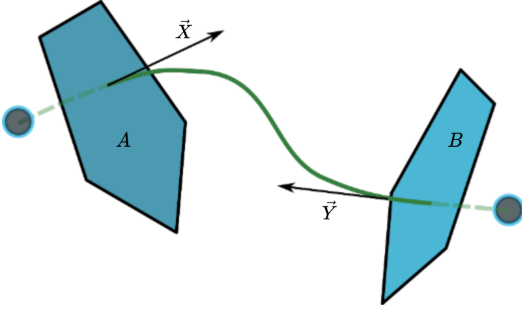
FIG. 5. The normal vectors to the faces at each end of an edge in terms of the spinors attached to each end.
