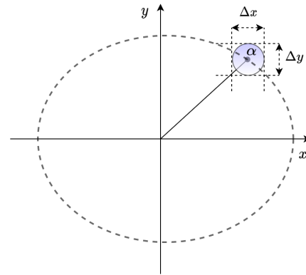
FIG. 1. The parameter \alpha which labels the coherent state |\alpha\rangle encodes the phase space co-ordinates of an ordinary classical oscillator. Time-evolution of the coherent state under the Schrödinger Hamiltonian yields a trajectory for \alpha which is precisely that of the classical oscillator.
