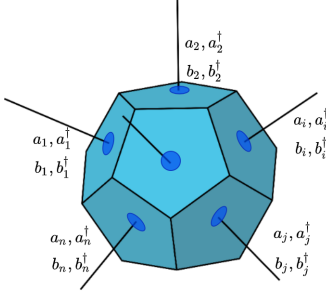
FIG. 8. Applying the Schwinger boson trick to each spin label on all the edges.
