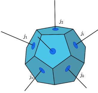
FIG. 3. An example of a spin-network vertex, with the associated polyhedron. The faces of the polyhedron are transverse to the edges attached to the vertex. The vertex itself lies in the interior of the polyhedron. Each edge punctures one of the faces and assigns it a quantum of area depending on the spin rep labelling the edge.
