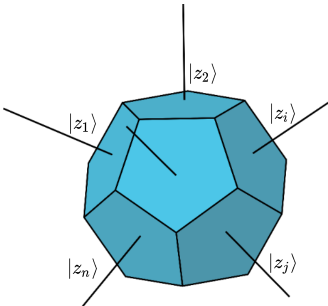
FIG. 6. The classical phase space of an intertwiner. Each leg is labelled by a spinor |z_i\rangle \in \mathbb{C}^2 where i \in \{1, \dots, n\} .
