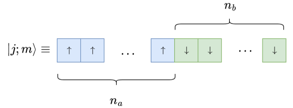
FIG. 2. Angular momentum state |j; m\rangle can be mapped to a system of 2j spin 1/2 particles.
