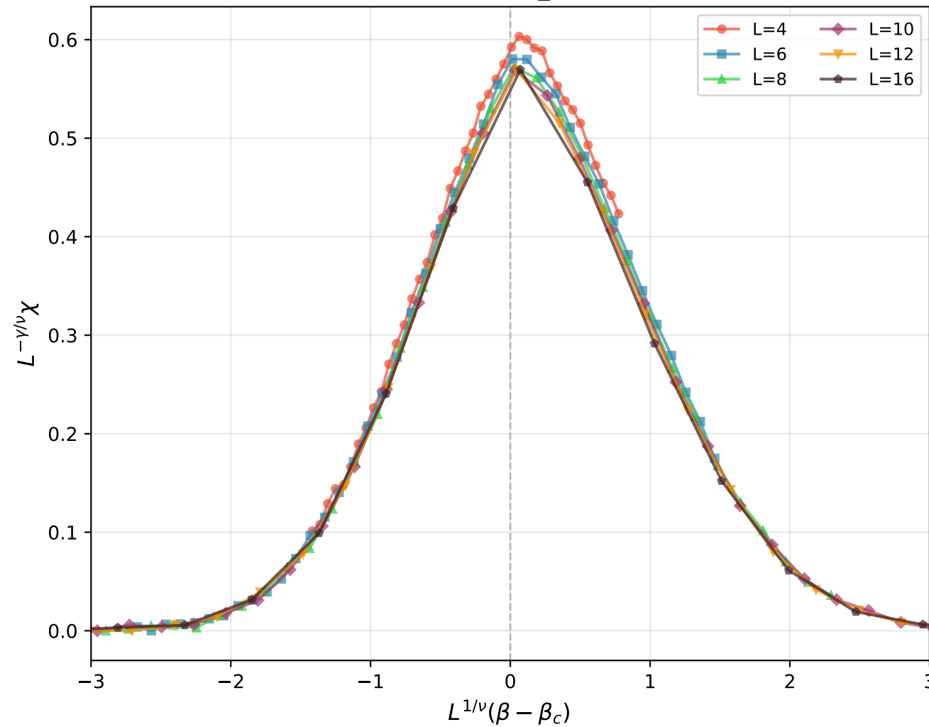
(a) Susceptibility Collapse \nu=0.639 , \beta_c=0.7616
