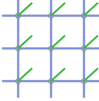
Figure 12: A spin-network as a tensor network whose “physical” degrees of freedom correspond to the allowed intertwiner states of four-valent vertices.
