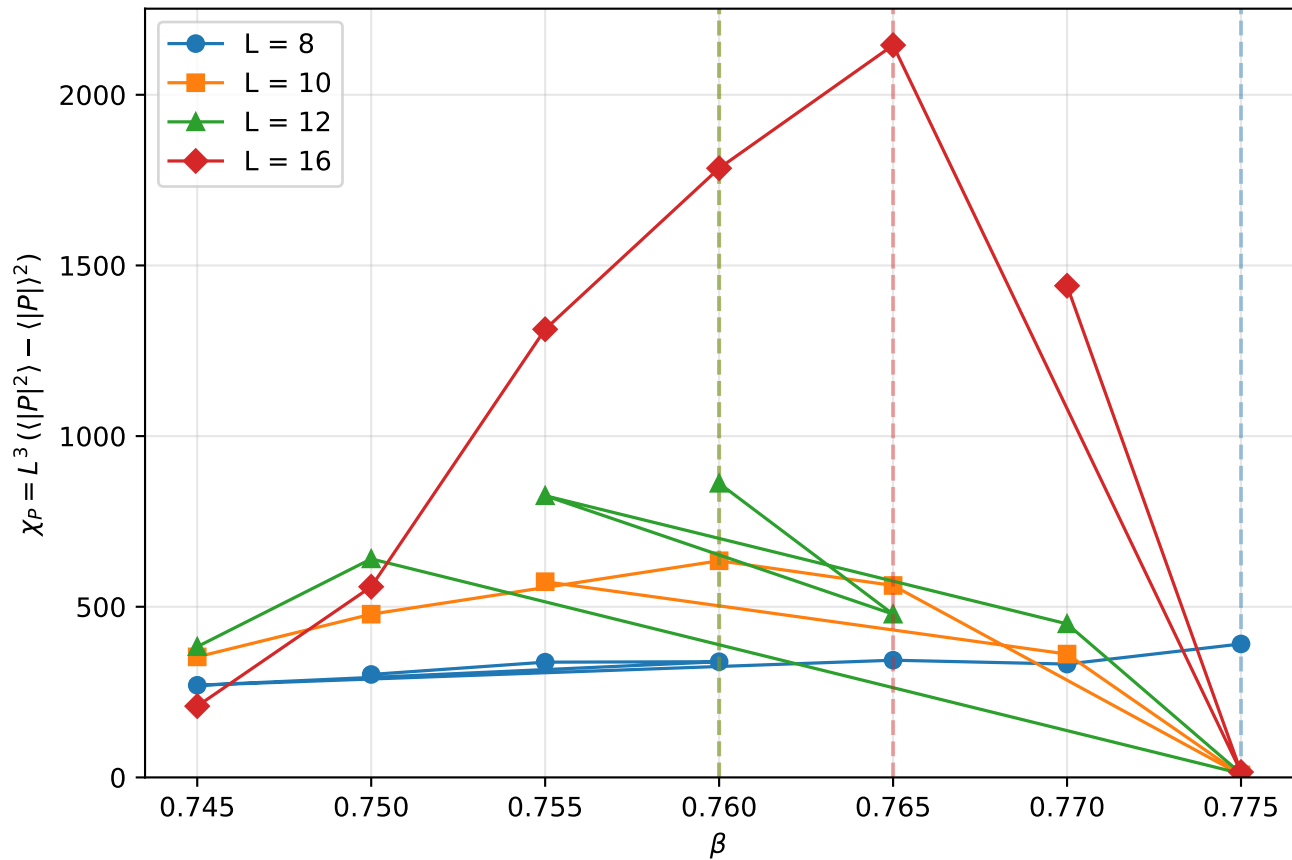
Polyakov Loop Susceptibility — Proof of Principle
