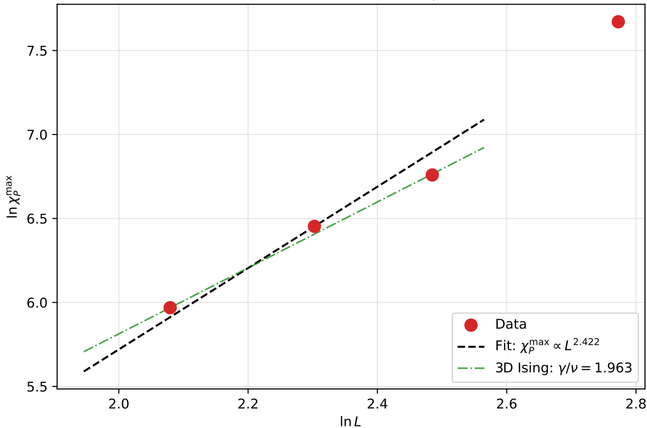
Peak Susceptibility Scaling: \chi_p^{\max} \propto L^{\gamma/\nu}
