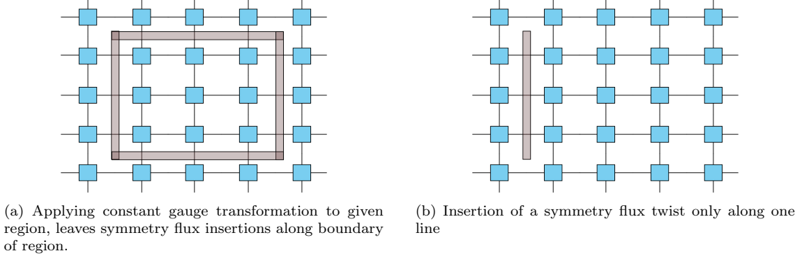
Figure 9: Local symmetry flux insertions in a 2D MPS
