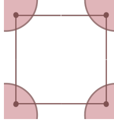
Figure 18: Each plaquette is in an entangled state: |0000\rangle + |1111\rangle
