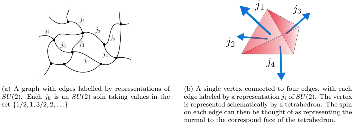
Figure 10: States of quantum geometry represented by spin-networks
