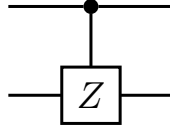
(a) The controlled Z gate. This and other quantum circuits were drawn using the Quantikz package by Alastair Kay [43]
