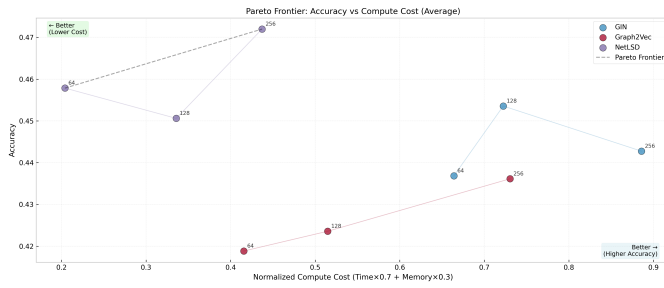
Figure 15: After permutation: Pareto frontier
