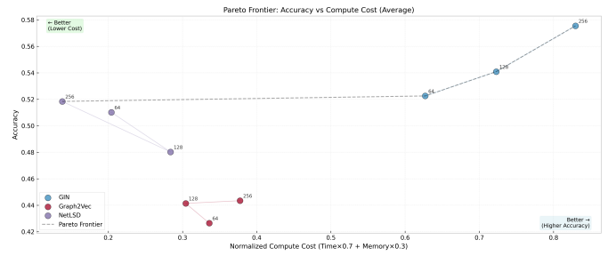
Figure 3: Pareto frontier illustrating the trade-off between accuracy and normalized compute cost.
