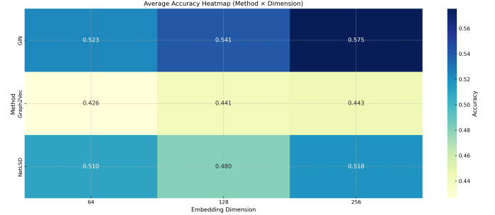
Fig. 1: Average accuracy heatmap across methods and embedding dimensions.
