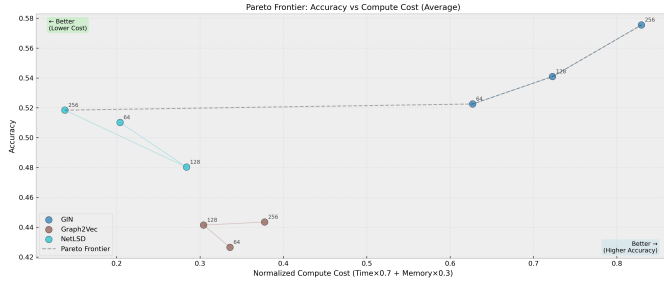
Fig. 2: Pareto frontier illustrating the trade-off between accuracy and normalized compute cost.
