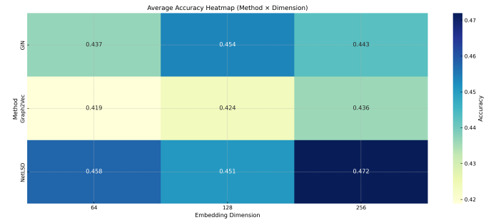
Figure 15: After permutation: average accuracy heatmap across methods and embedding dimensions.
