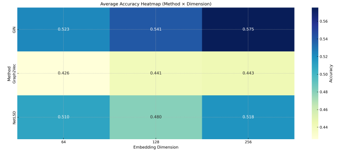
Figure 2: Average accuracy heatmap across methods and embedding dimensions.
