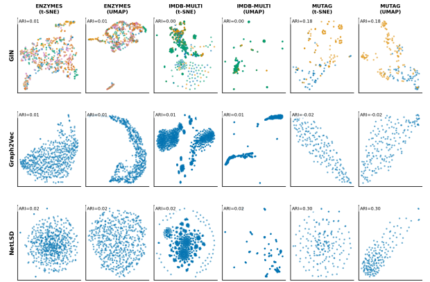
Figure 14: t-SNE vs UMAP Clusters Comparison across algorithms and datasets The dimensionality reduction technique greatly influences cluster visualization.
