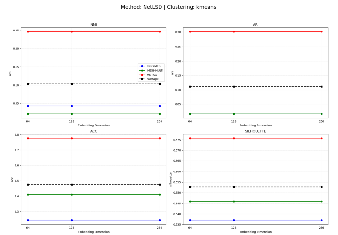
Fig. 7: NetLSD K-Means Performance. It outperforms others in stability.
