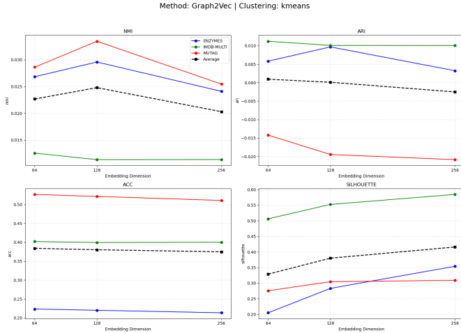
Fig. 8: Graph2Vec K-Means Performance.
