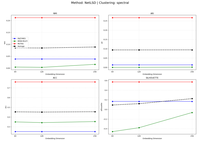
Fig. 10: NetLSD Spectral Clustering. The trend mirrors K-Means.
