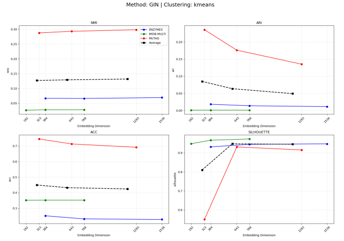
Fig. 9: GIN K-Means Performance.
