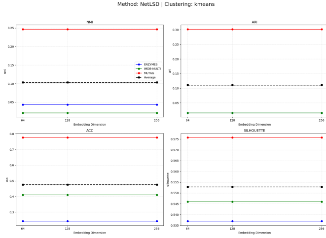
Fig. 7: NetLSD K-Means Performance. It outperforms others in stability.
