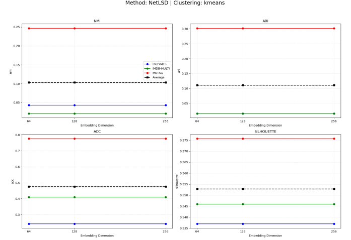
Fig. 6: NetLSD K-Means Performance. It outperforms others in stability.
