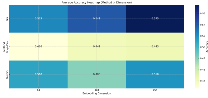
Fig. 1: Average accuracy heatmap across methods and embedding dimensions.
