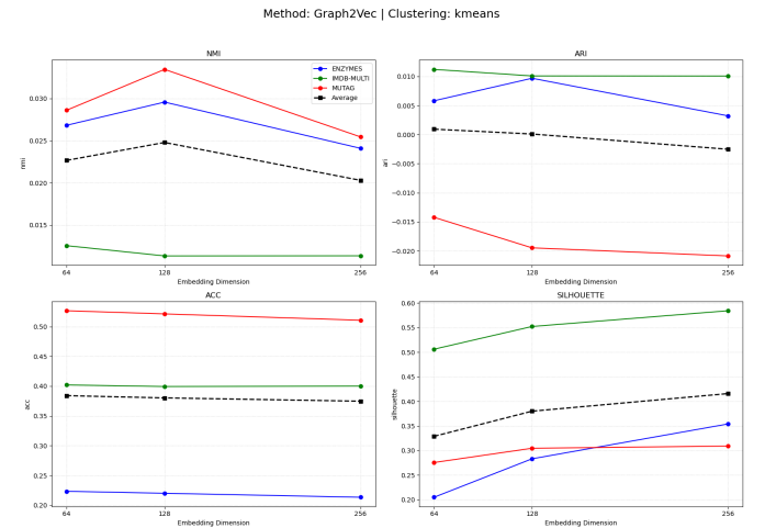
Fig. 7: Graph2Vec K-Means Performance.
