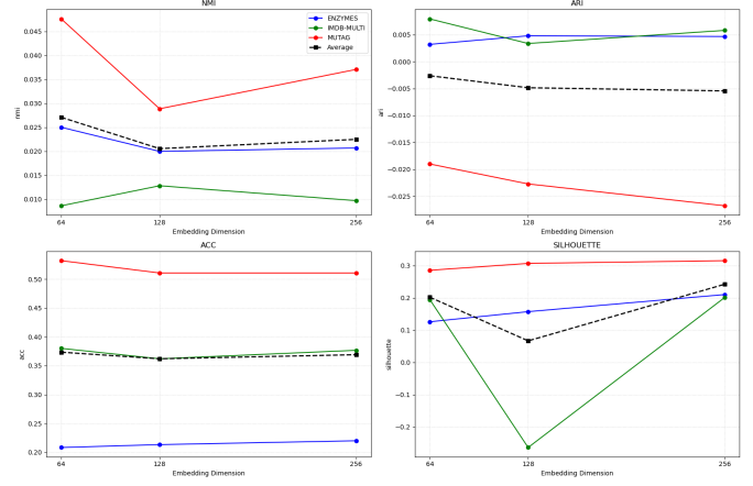
Fig. 10: Graph2Vec Spectral Clustering.
