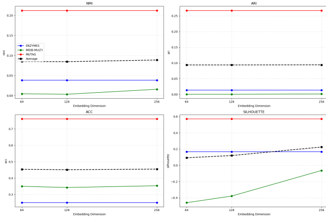
Fig. 9: NetLSD Spectral Clustering. The trend mirrors K-Means.
