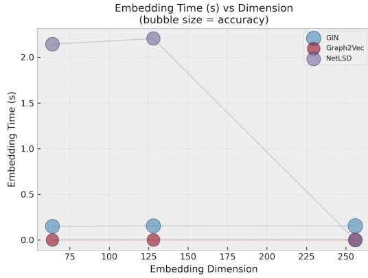
Fig. 3: Embedding time as a function of embedding dimension.
