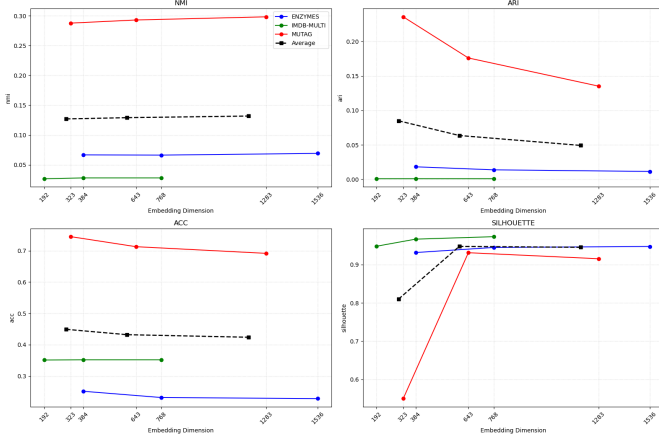
Fig. 8: GIN K-Means Performance.
