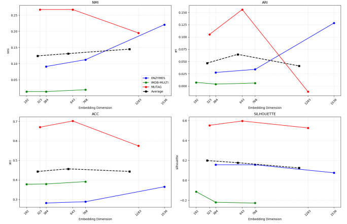
Fig. 11: GIN Spectral Clustering. Consistently mirrors structural properties.
