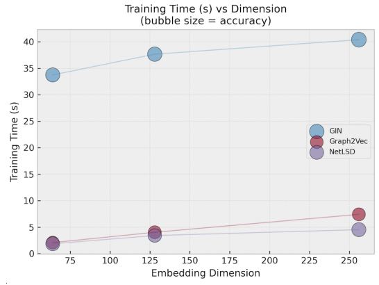
Fig. 4: Training time as a function of embedding dimension.
