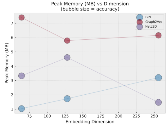
Fig. 5: Peak memory usage as a function of embedding dimension.
