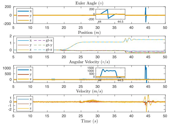
Fig. 11. Attitude, position, angular velocity, and linear velocity in the UAV flip experiment. The notation “gt” stands for the position ground truth collected by a VICON motion capture system.
