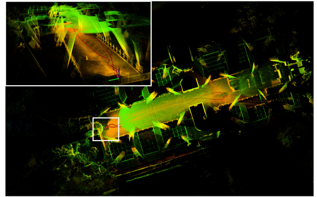
Fig. 12. Mapping results of FAST-LIO2 in the fast motion handheld experiment.
