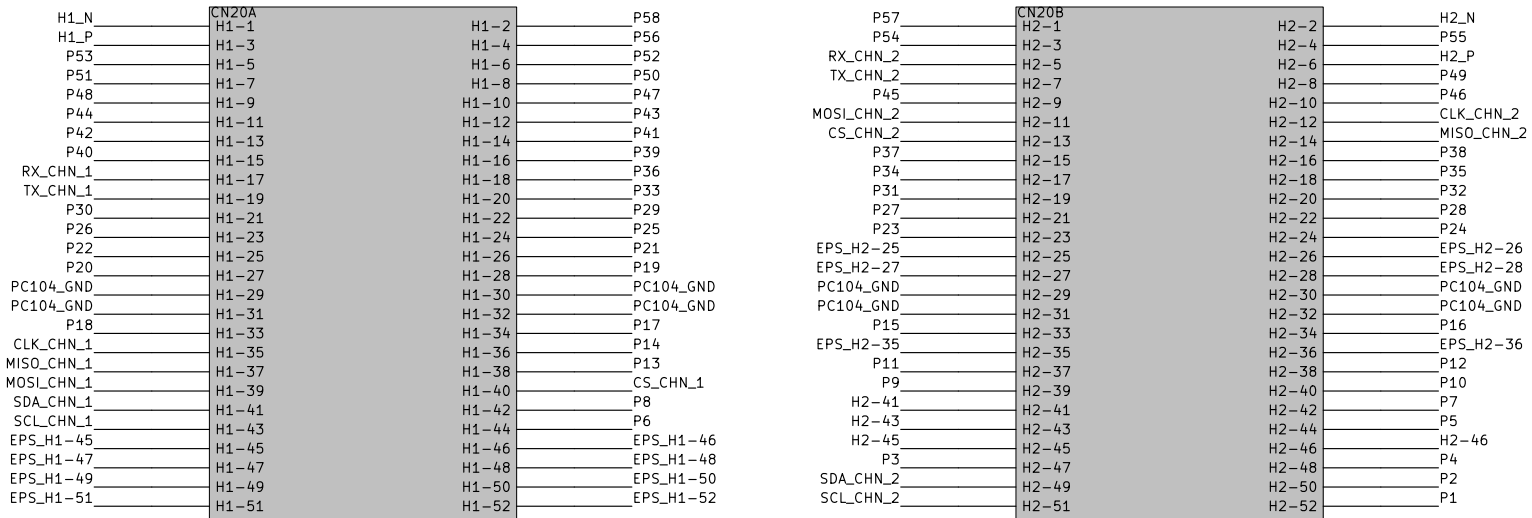
PC104 slot N°1 (EPS)
