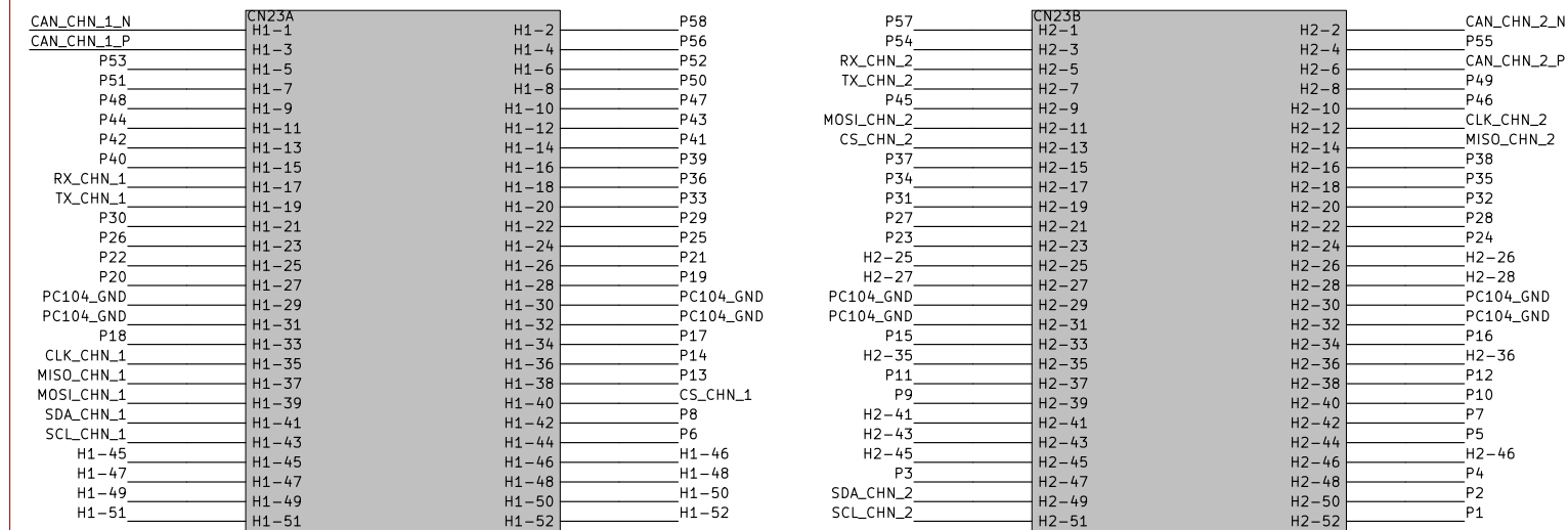
PC104 slot N°2 (CAN bus tests)
