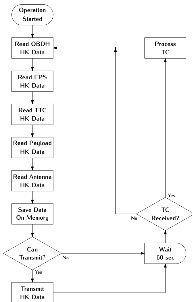
Figure 2.8: Transmit/Receive flowchart
