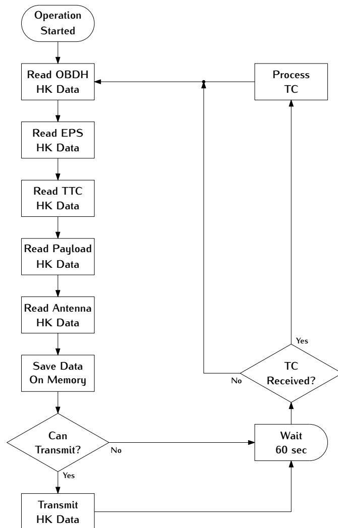
Figure 2.8: Transmit/Receive flowchart
