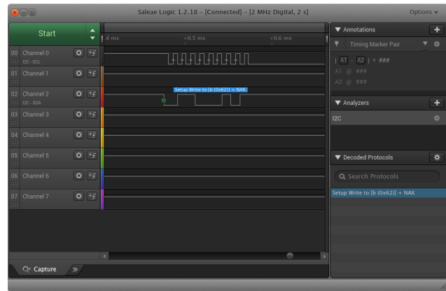
(b) Waveforms of the I 2 C port 2 test.
