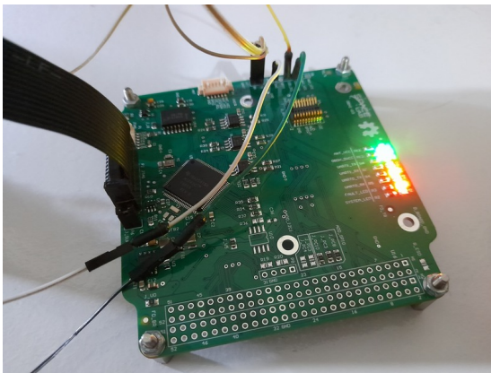
(a) Connections of the I 2 C port 2 test.
