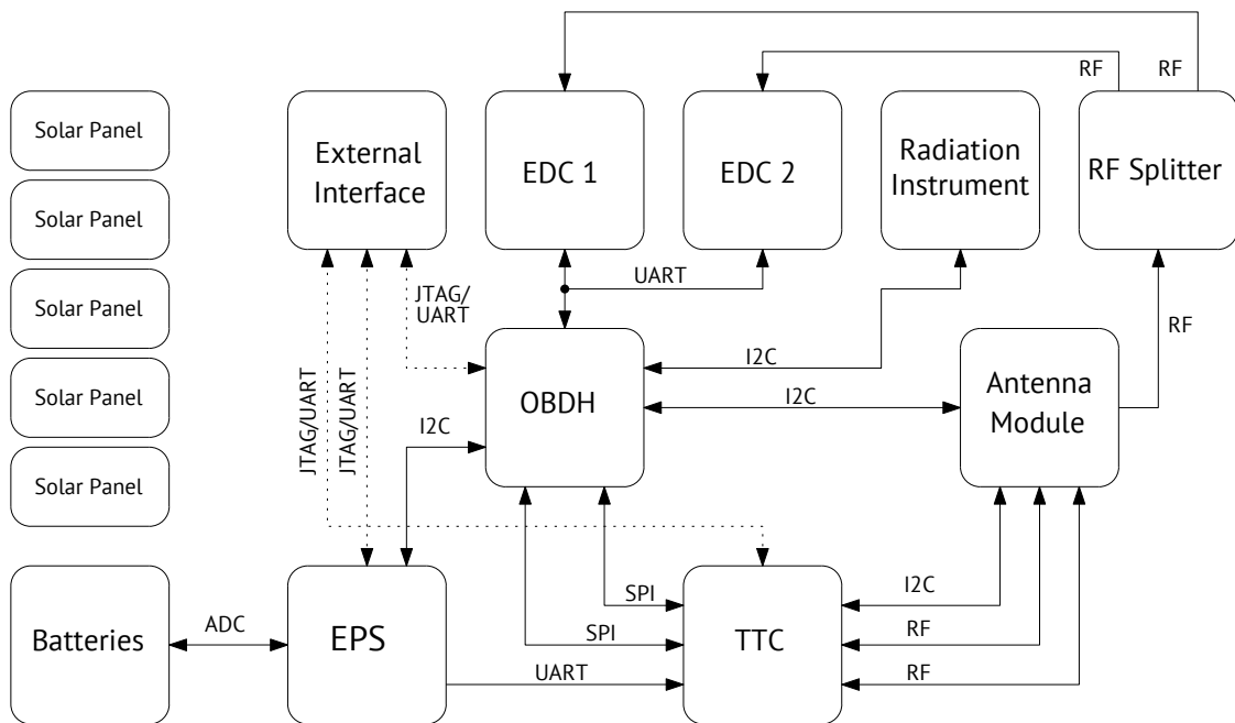
Figure 2.8: Data path diagram.
