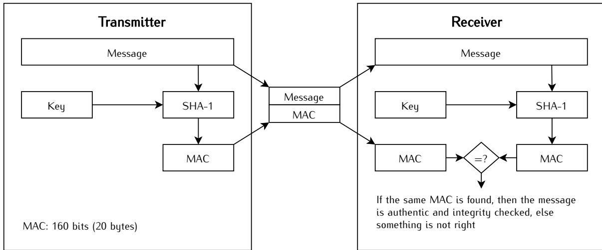
Figure 4.3: Diagram of the used HMAC scheme.
