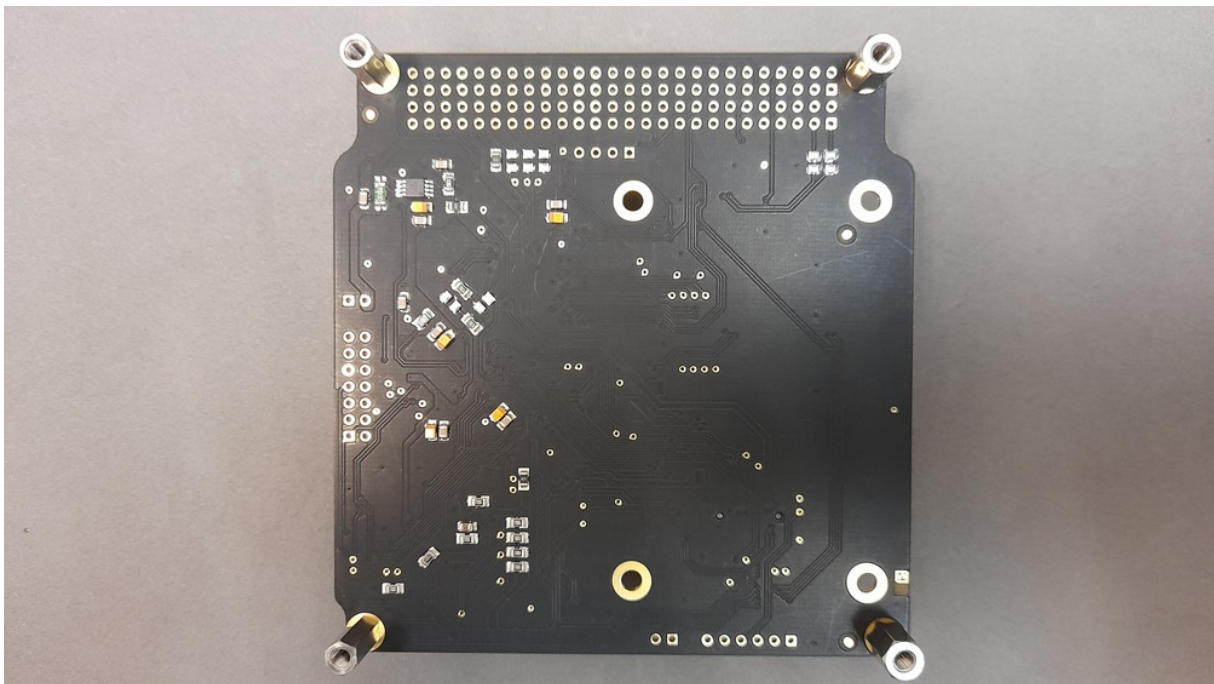
Figure D.2: Bottom view of the OBDH 2.0 v0.7 board.
