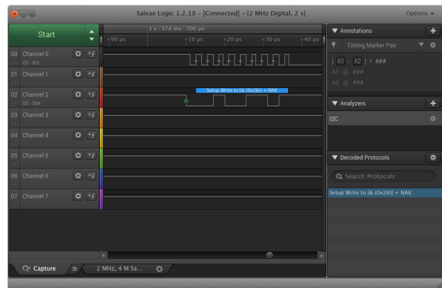
(b) Waveforms of the I 2 C port 0 test.
