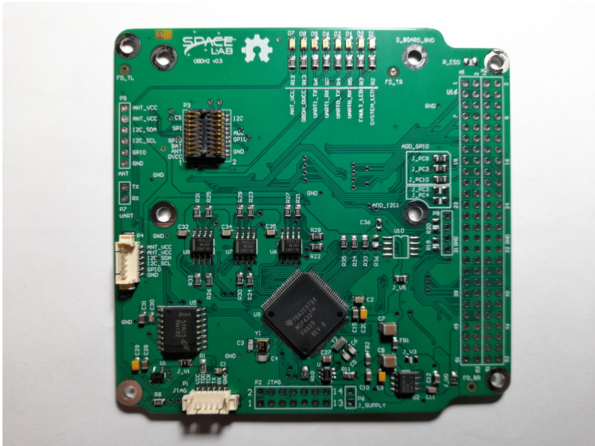
Figure C.1: Top view of the OBDH 2.0 v0.5 board.
