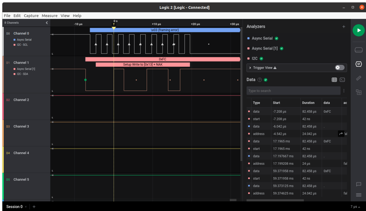
Figure D.5: Waveform of the I2C port 0.
