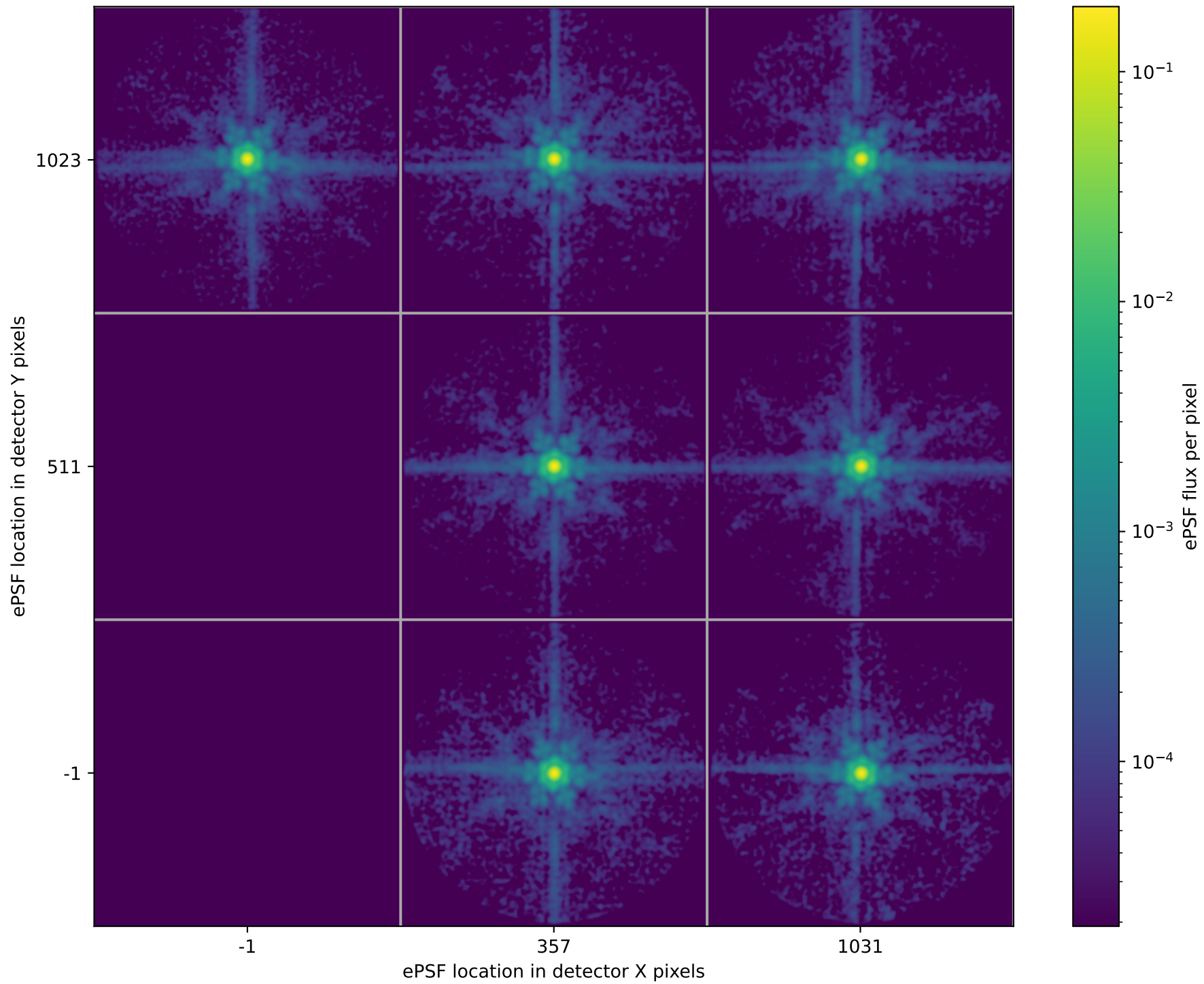
MIRI F560W ePSFs
