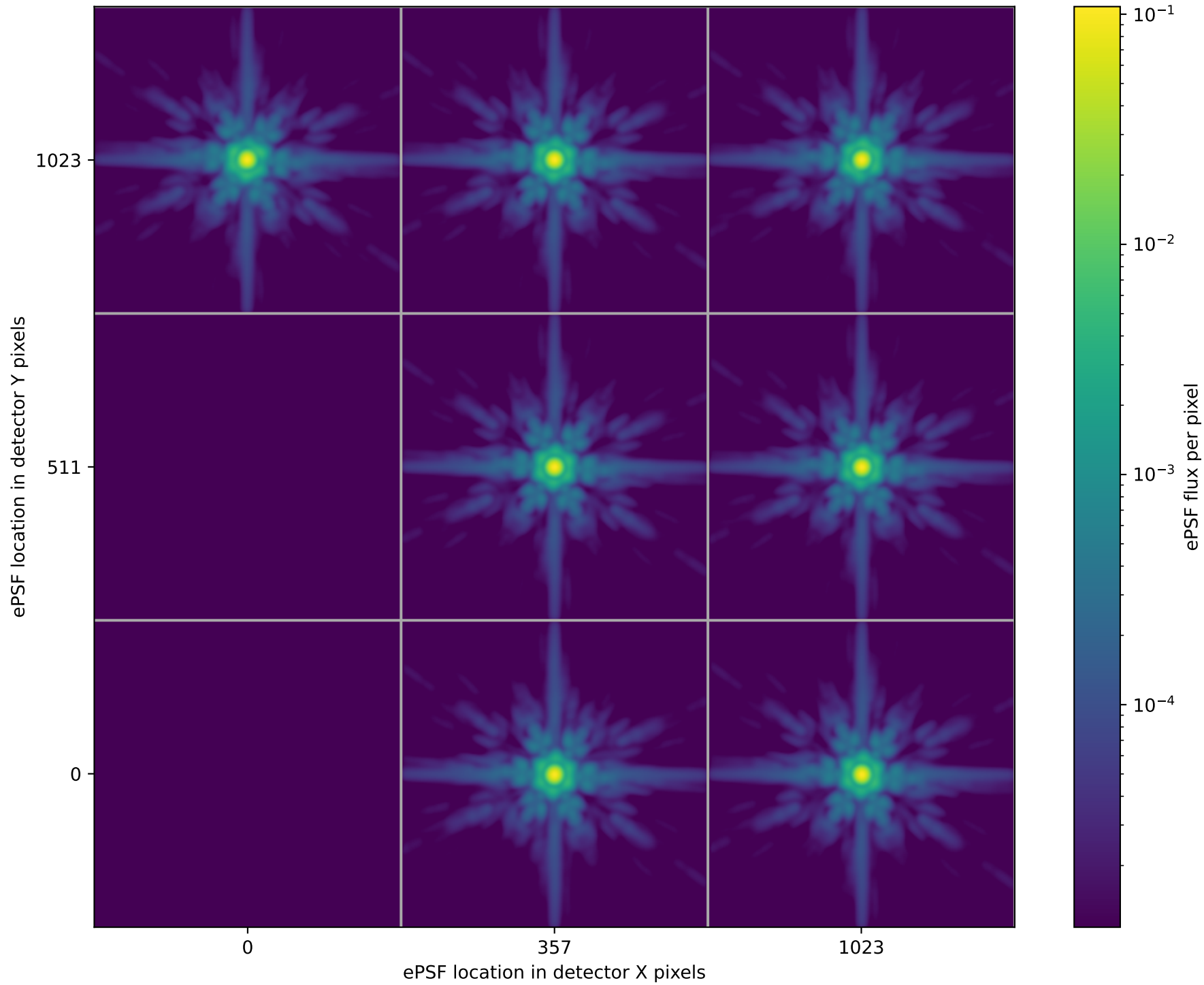
MIRI MIRIM F770W ePSFs
