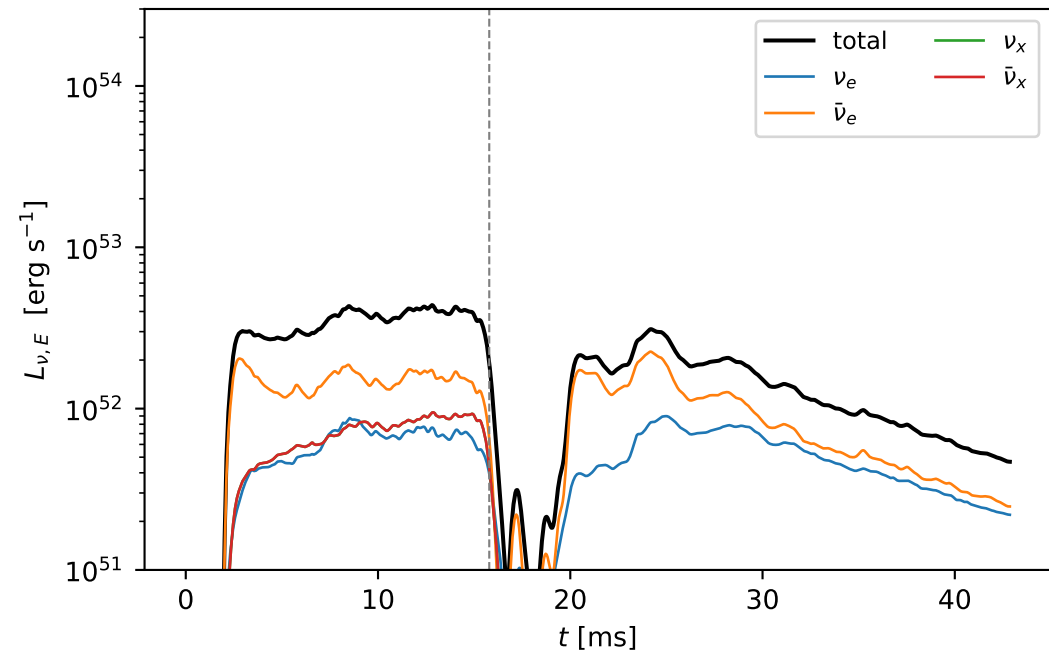
Energy luminosity
