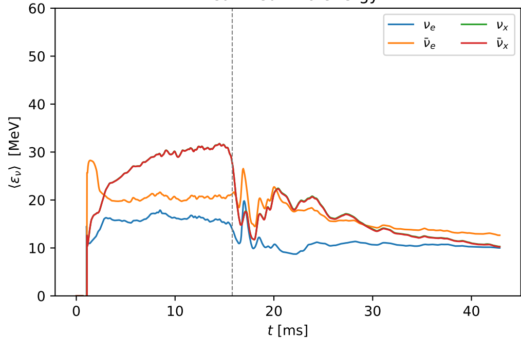
Mean neutrino energy
