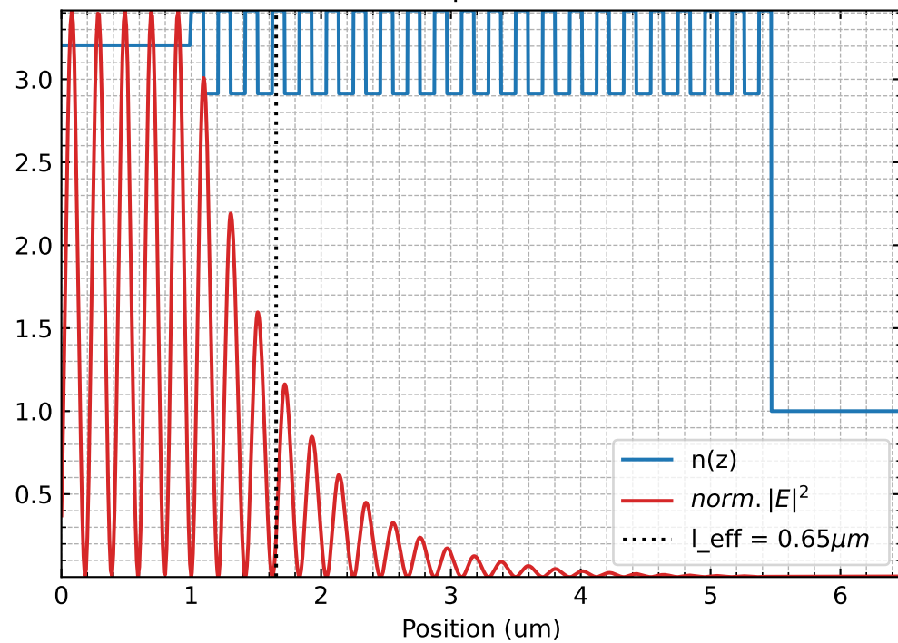
Top DBR
