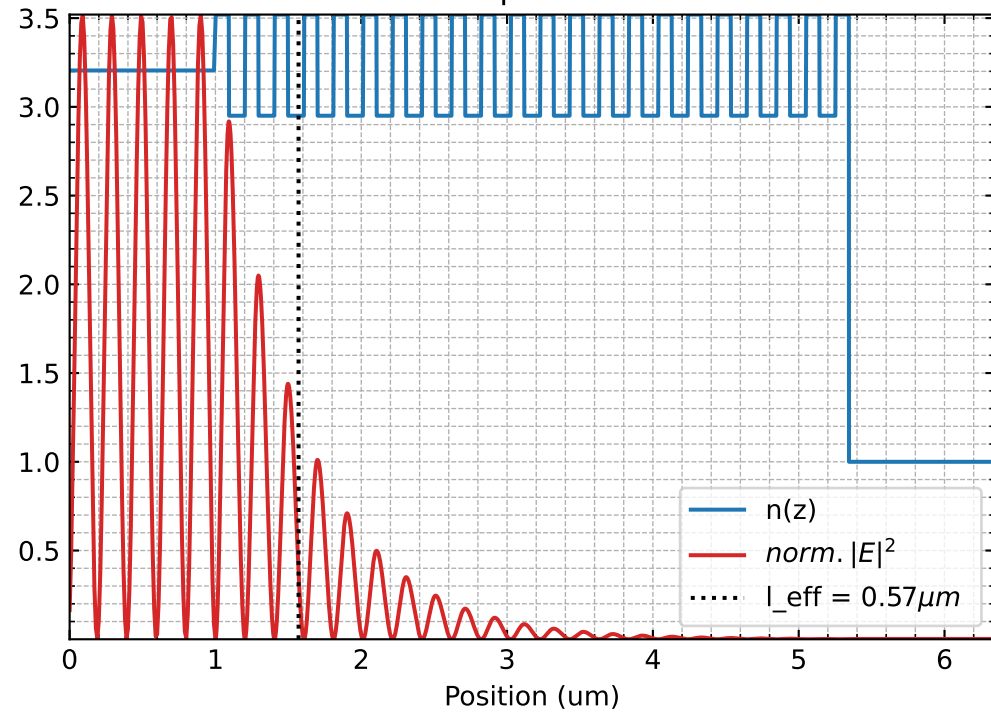
Top DBR
