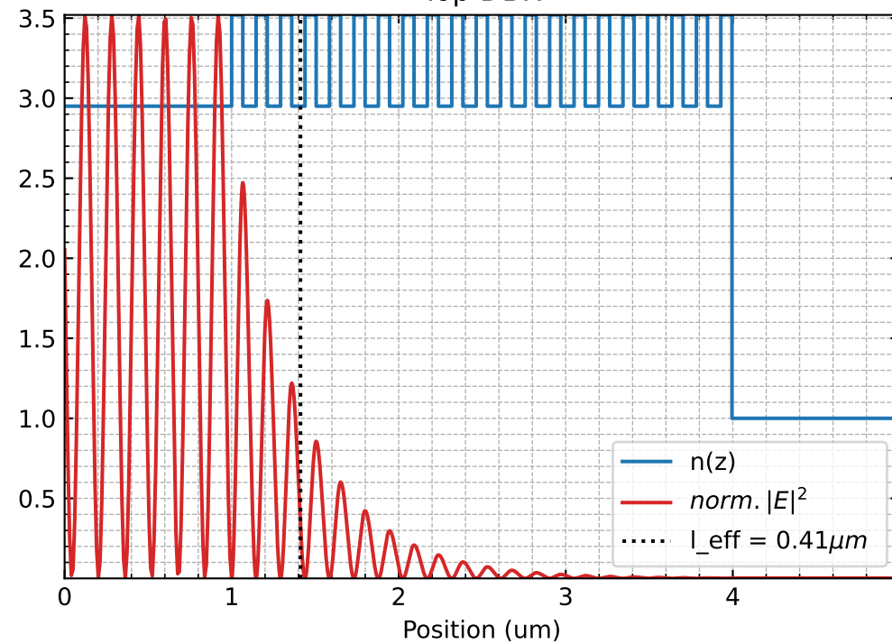
Top DBR
