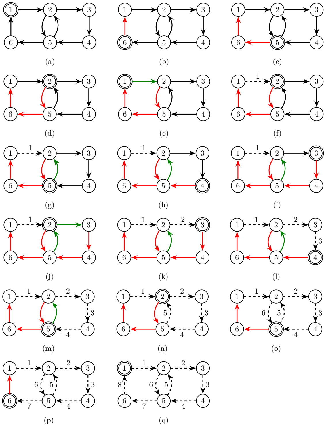
Figure 3.1: Sample execution of SPACE-EFFICIENT-HIERHOLZER. For clarity, DASHED edges are labelled in the order in which they are written. The current vertex is represented by double borders.
