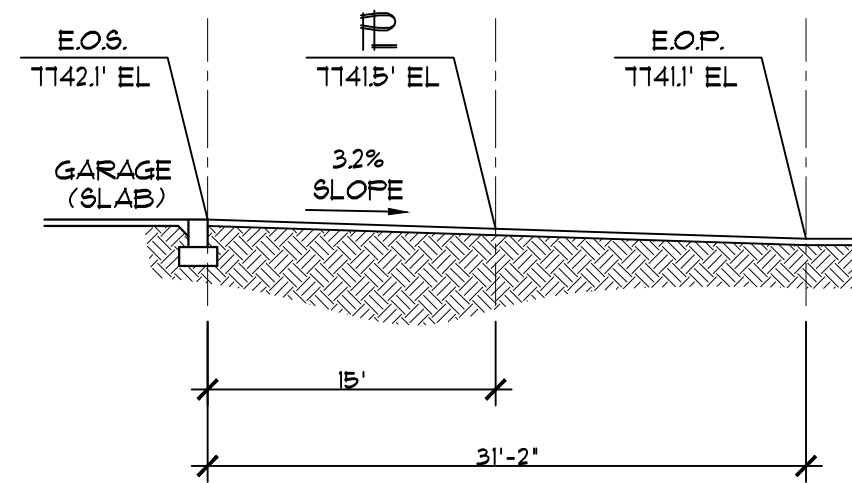
DRIVEWAY PROFILE SCALE: 1"=10'
