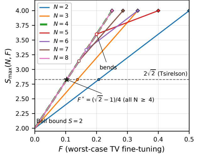
FIG. 1. Exact curves S_{\max}(N, F) for N = 2, \dots, 8 (Theorem 5), computed in exact rational arithmetic from Eq. (7). The N = 4 and N = 8 curves coincide ( 2 + 8F up to F = \frac{1}{4} , then 4); the N = 4 curve is drawn dashed so that both remain visible. Every curve starts at the Bell value S = 2 with initial slope 2\min(N, 4) . Open circles mark the bends at F = 1/N for N = 5, 6, 7 , where rows of the maximizing multiset exhaust their wrong-sign states and the slope drops; diamonds mark the caps F(S=4; N) = \lfloor N/4 \rfloor / N (Eq. (11)), beyond which each curve is flat at S = 4 . The star marks the saturation value F^* = (\sqrt{2} - 1)/4 , at which all curves with N \geq 4 cross the Tsirelson value 2\sqrt{2} (dashed line); the dots are the N = 2, 3 crossings.
