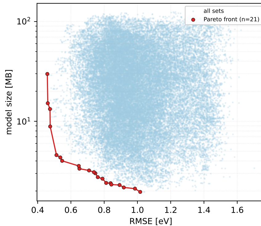
RMSE vs model size (Spearman \rho=-0.07 )
