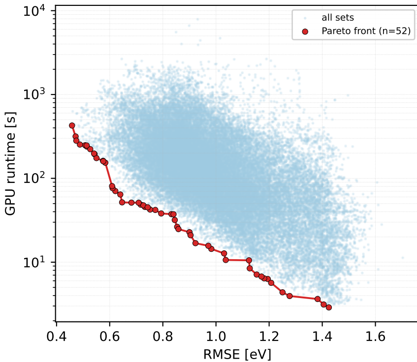
RMSE vs GPU runtime (Spearman \rho=-0.61 )
