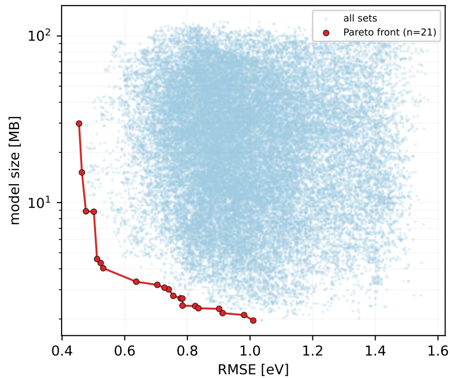
RMSE vs model size (Spearman \rho=-0.08 )
