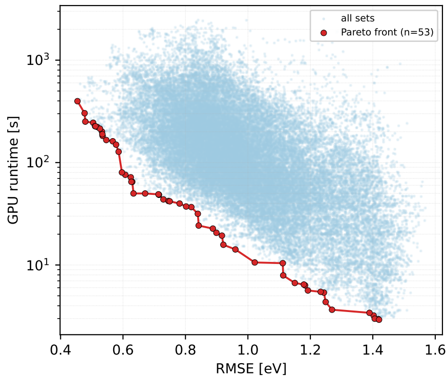
RMSE vs GPU runtime (Spearman \rho=-0.62 )
