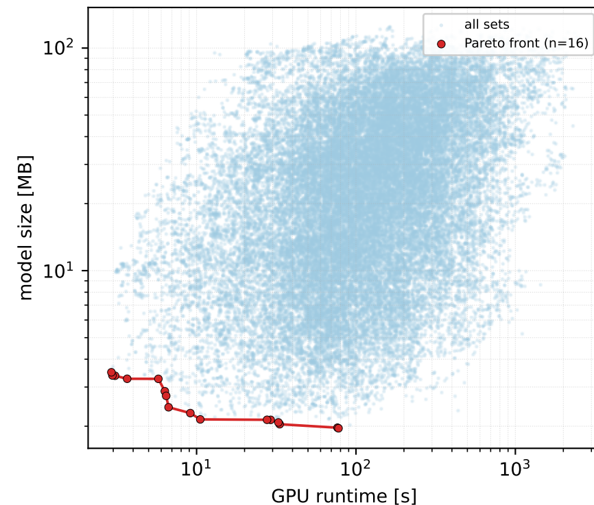
GPU runtime vs model size (Spearman \rho=0.38 )
