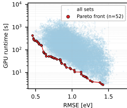
RMSE vs GPU runtime (Spearman \rho=-0.61 )
