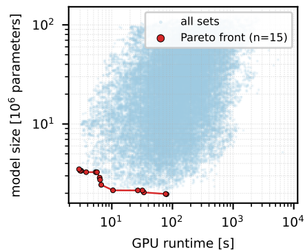
GPU runtime vs model size (Spearman \rho=0.3 )
