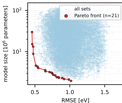
RMSE vs model size (Spearman \rho=-0.07 )
