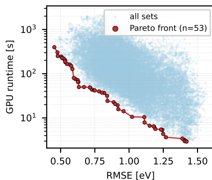
RMSE vs GPU runtime (Spearman \rho=-0.62 )
