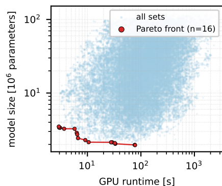
GPU runtime vs model size (Spearman \rho=0 )
