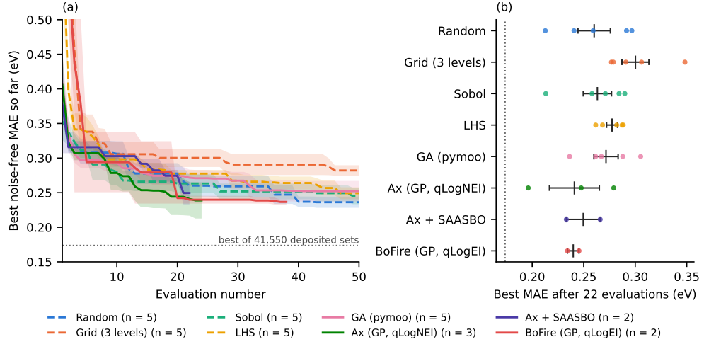
Fig. 5 Optimization strategies on the released surrogate (minimize MAE, train_frac = 1, noisy observations). (a) Best noise-free MAE found so far (surrogate at median noise rank) against the number of evaluations, averaged over repeated campaigns ( n in the legend; shaded band: standard error). Dashed lines are non-adaptive designs and solid lines adaptive methods; Ax, Ax with SAASBO, and BoFire curves end at the last evaluation reached by all of their campaigns (24, 22, and 38). (b) Best noise-free MAE after 22 evaluations, the largest budget reached by every method; dots are individual campaigns and bars show the mean and standard error. The dotted line marks the best of the 41,550 deposited hyperparameter sets.
