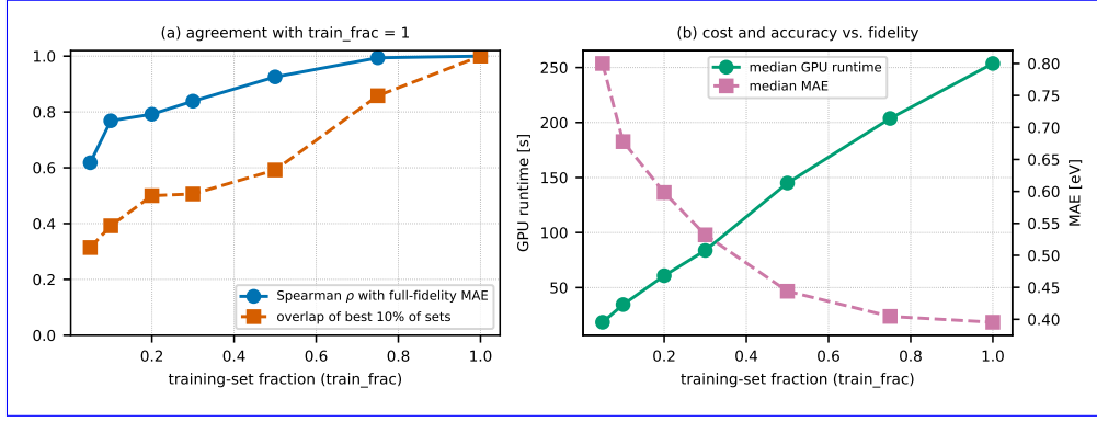
Fig. 3 The training-set fraction as a fidelity parameter, from surrogate predictions (median noise rank) for 5,000 deposited hyperparameter sets. (a) Spearman correlation between MAE at a given train_frac and MAE at train_frac = 1 , and overlap of the best 10% of sets. (b) Median GPU runtime and median MAE as a function of train_frac .
