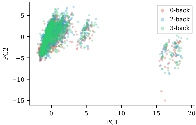
Algo-1: Statistical+Spectral (52-d) Var explained: 27.4%
