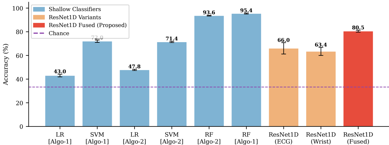
5-Fold CV Performance Comparison — All Models
