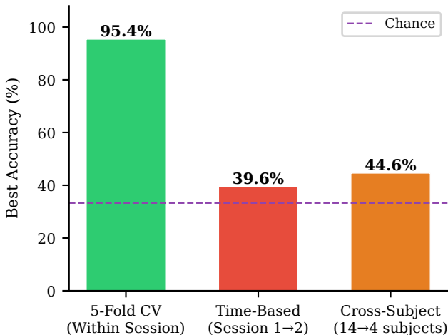
Performance vs. Evaluation Protocol (Best model per protocol)
