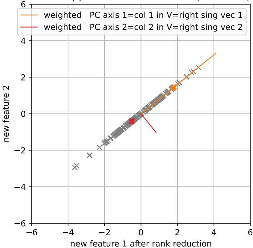
rank-1 approximation of 2D data (line in 2D)
