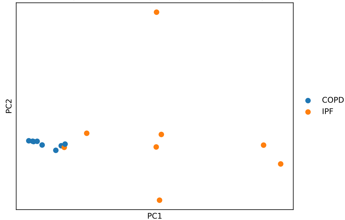
PCA of psuedobulk samples - T cells (Low quality)
