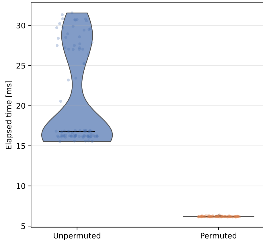
CPU kernel runtime (R02B05)
