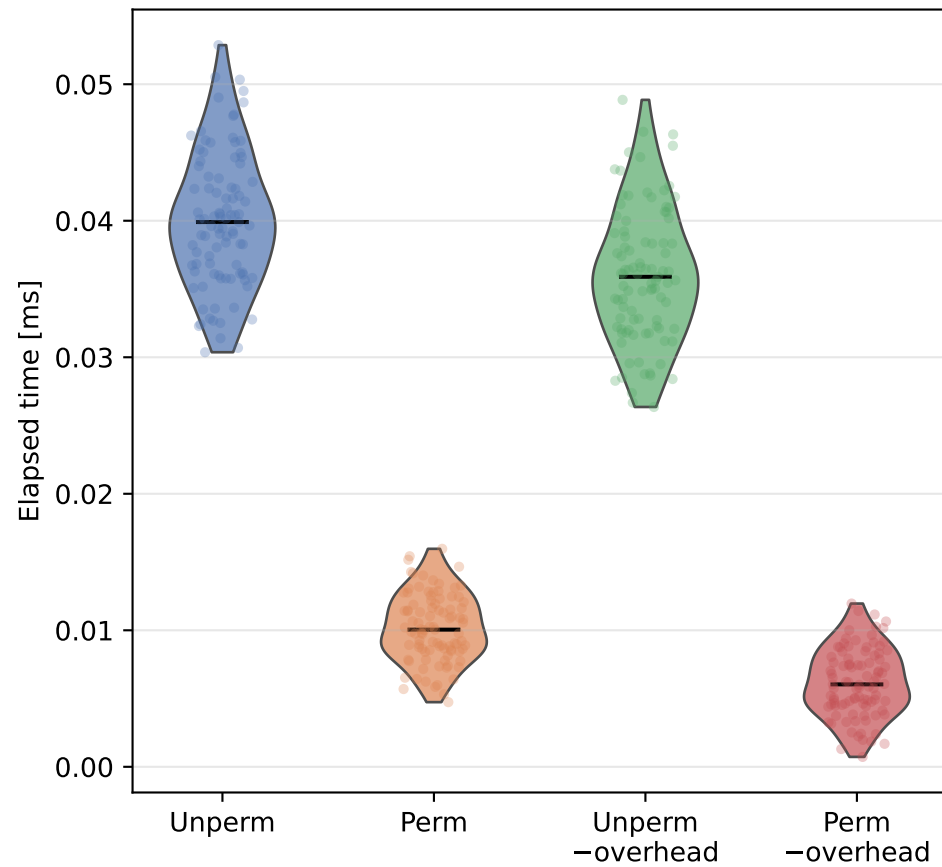
GPU kernel runtime (R02B05)
