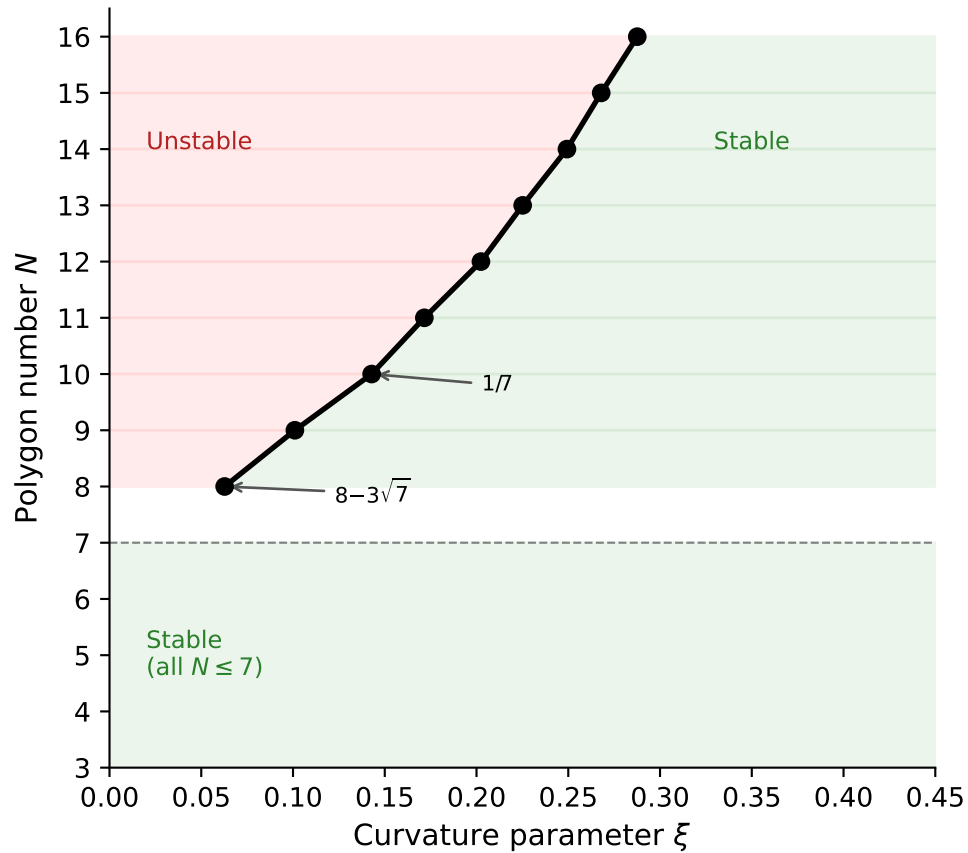
H 2 : Stability boundary
