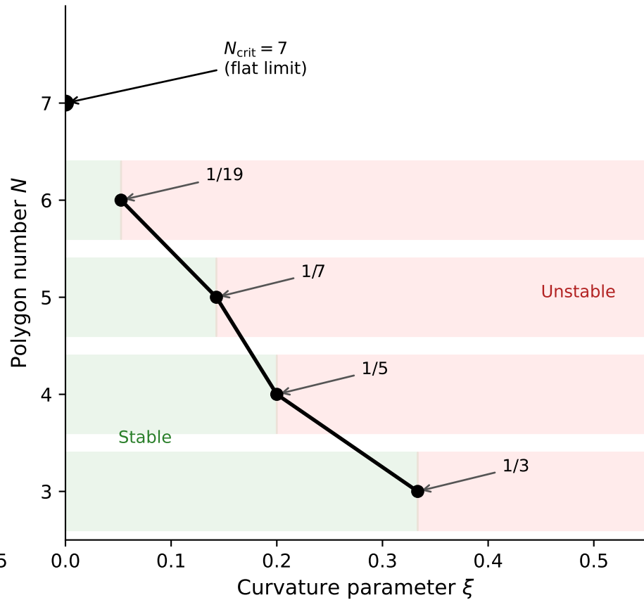
S 2 : Stability boundary
