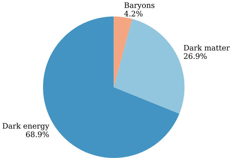
Theory ( N = 11 )
