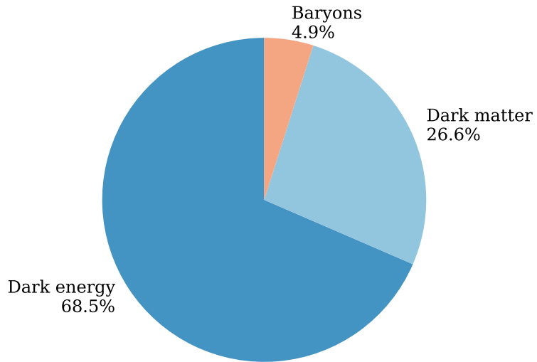
Planck 2018
