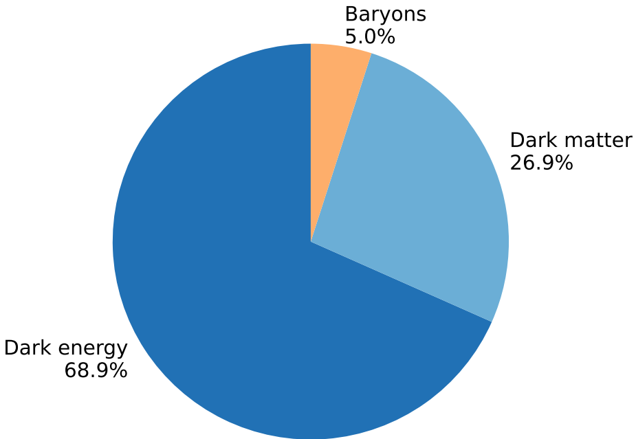
Theory ( N = 11 )
