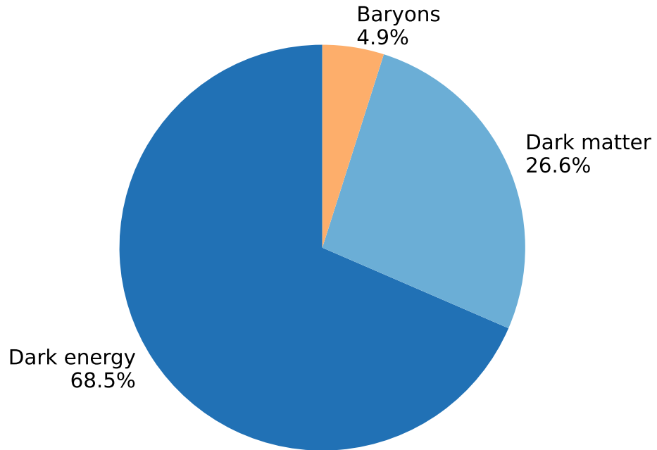
Planck 2018
