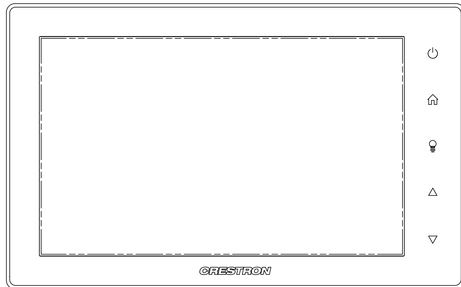
2 TPL2 CRESTRON TSW-750-W-S SCALE: 1' = 1'-0"
