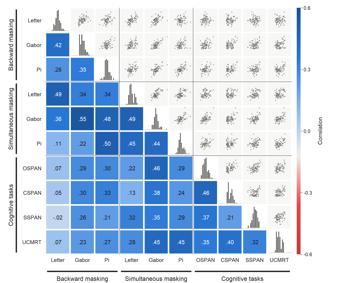
Figure 3. corr plot
