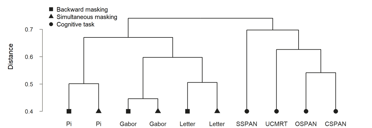
Figure 4. hcluster
