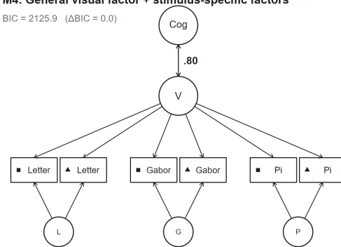
M4: General visual factor + stimulus-specific factors
