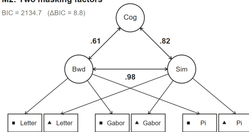
M2: Two masking factors
