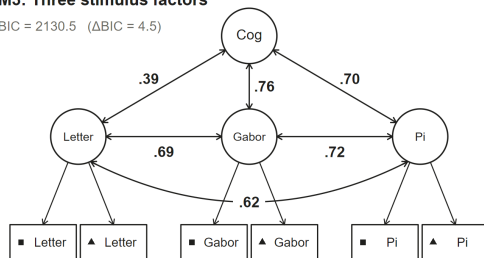
M3: Three stimulus factors
