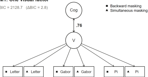
M1: One visual factor
