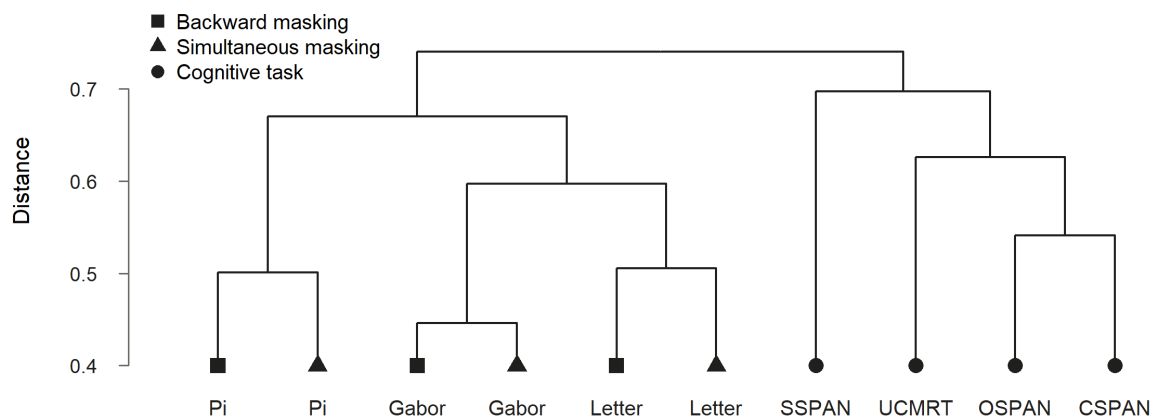
Figure 4. Hierarchical clustering of the ten tasks, based on the distance 1 - r between model-estimated correlations and average linkage. Symbols mark backward masking, simultaneous masking, and cognitive tasks.
