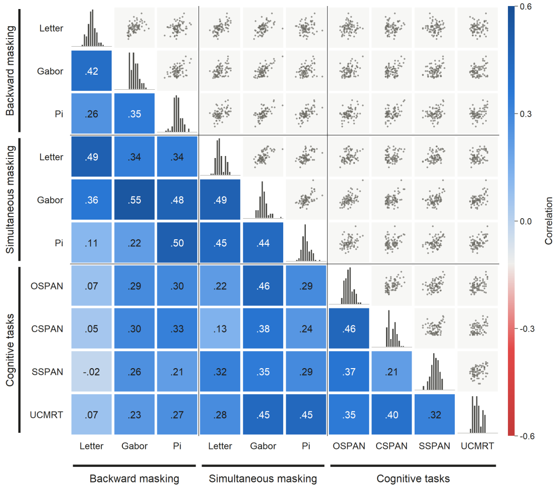
Figure 3. Model-estimated scores and correlations for the six masking tasks and the four cognitive tasks. Diagonal: distributions of the standardized scores. Lower triangle: model-estimated correlations. Upper triangle: scatterplots of the standardized scores.
